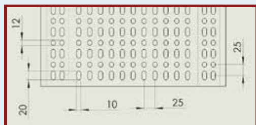
Perforation Detail
